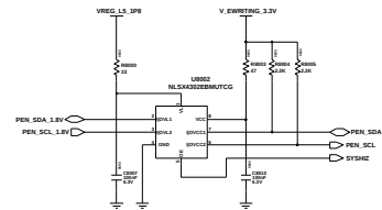
LEVEL SHIFTER
