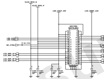
LCD Connector
