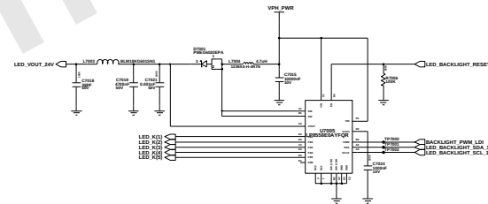
LCD BACKLIGHT DRIVER IC
