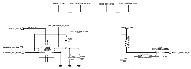
Accelerometer Sensor
