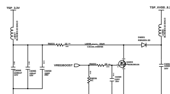
XVDD Booster Discrete
