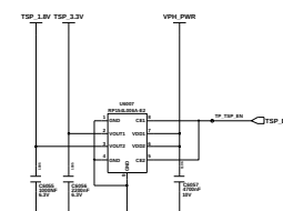
TSP Dual LDO
