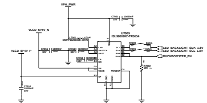
LCD BUCK BOOSTER
